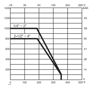
PTFE Ball Seat Pressure Temperature Rating
