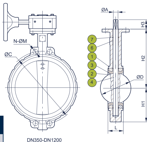
DN350-DN1200
